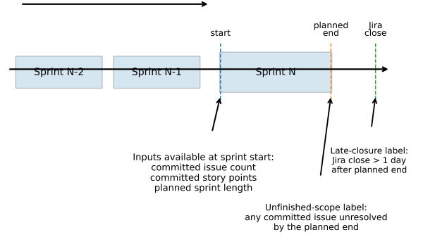
Fig. 1. Data timing and reconstruction used before model fitting.
