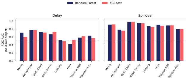
Fig. 2. Held-out-project AUC by project.
